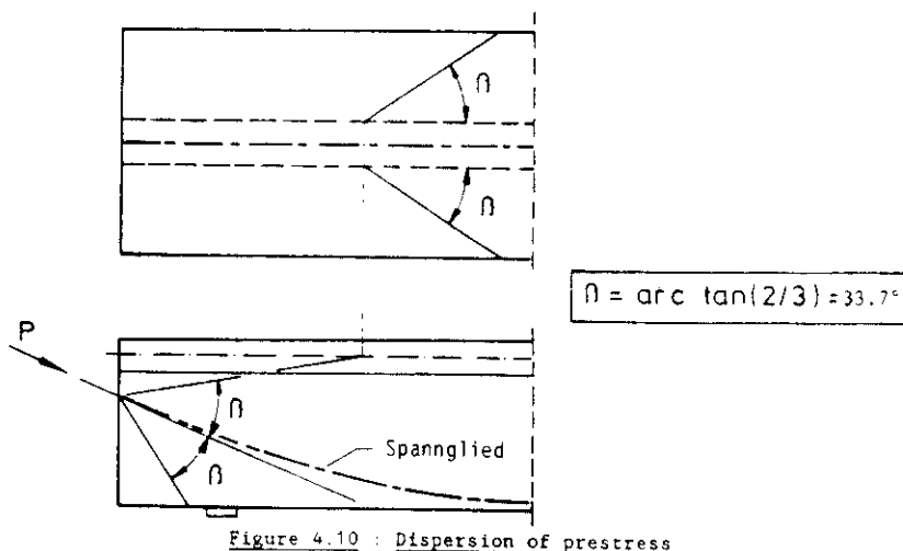
Figure 4.10 : Dispersion of prestress
