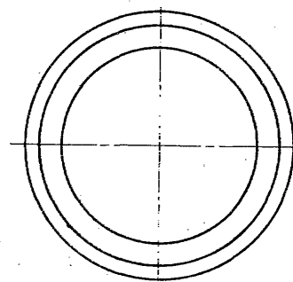
Tellerdübel System Christoph & Unmack
